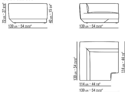
COD. 02D366 CORNER
