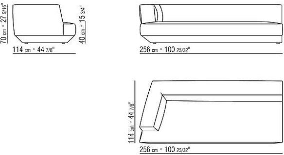
COD. 02D319 END UNIT L
