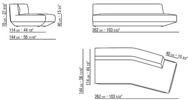
COD. 02D349 SIX SIDED TERMINAL UNIT L
