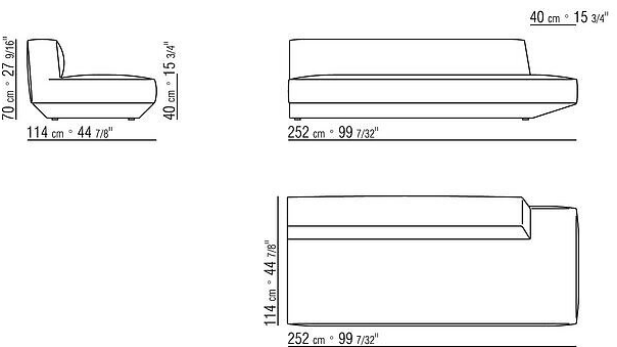
COD. 02D345 TERMINAL UNIT L
