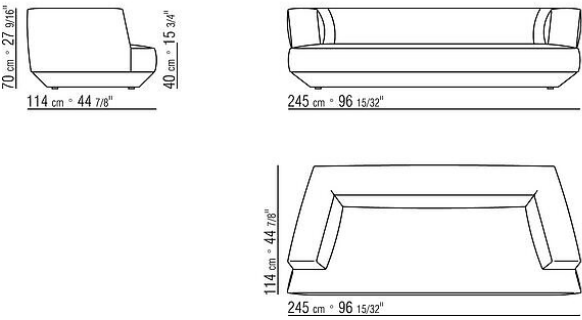
COD. 02D307 UNIT
