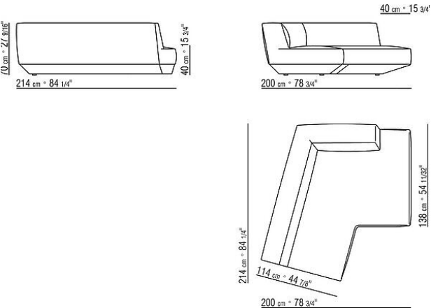
COD. 02D323 LONG CORNER L
