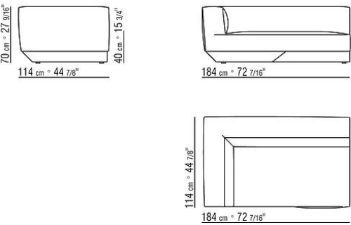
COD. 02D339 CORNER L
