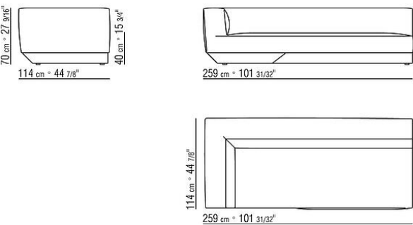
COD. 02D343 TERMINAL UNIT L
