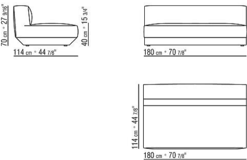
COD. 02D313 END UNIT L
