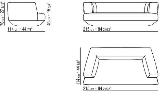
COD. 02D305 SOFA
