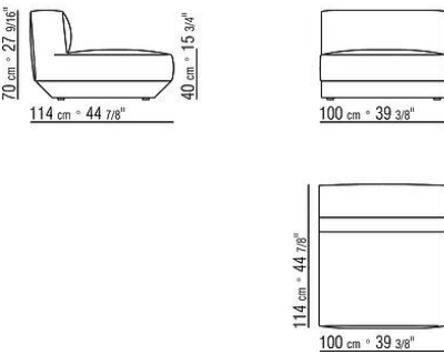
COD. 02D309 UNIT
