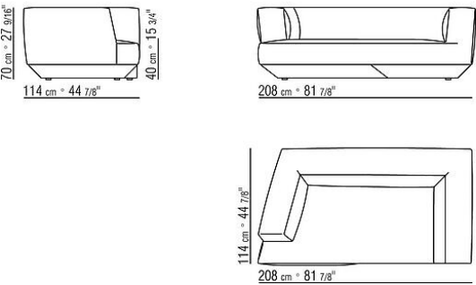
COD. 02D377 SIX SIDE SOFA / CORNER L
