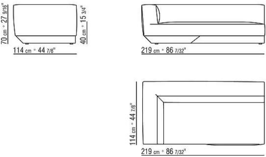
COD. 02D341 TERMINAL UNIT L
