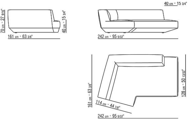
COD. 02D325 LONG CORNER L
