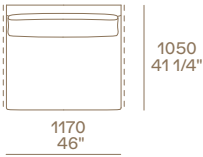
centrale central unit
